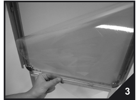
3. Insert them under the protective foil.
